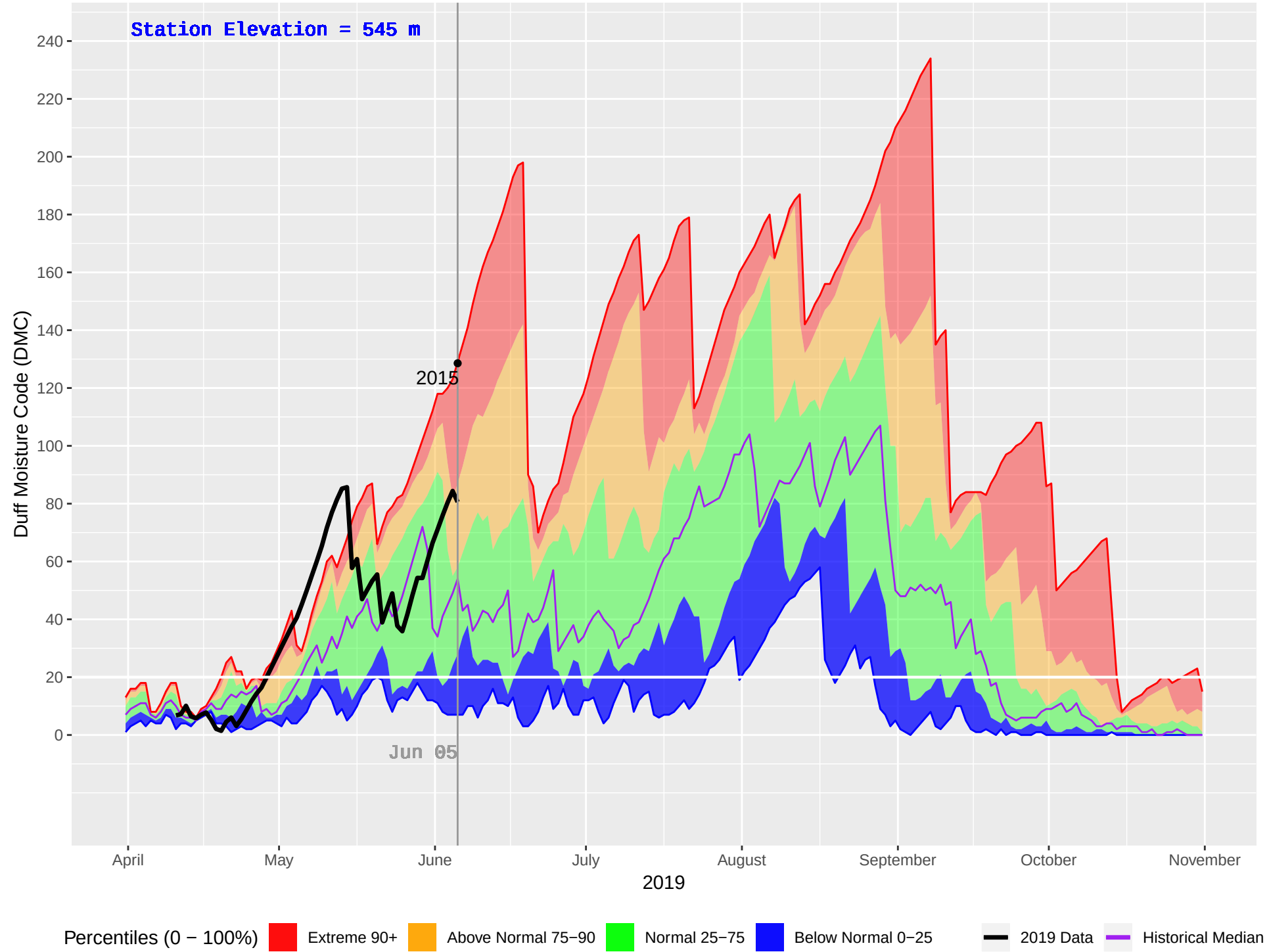
MEAGER CREEK (1083) : Historical (2010–2018), Current (2019) Daily Duff Moisture Code (DMC)
