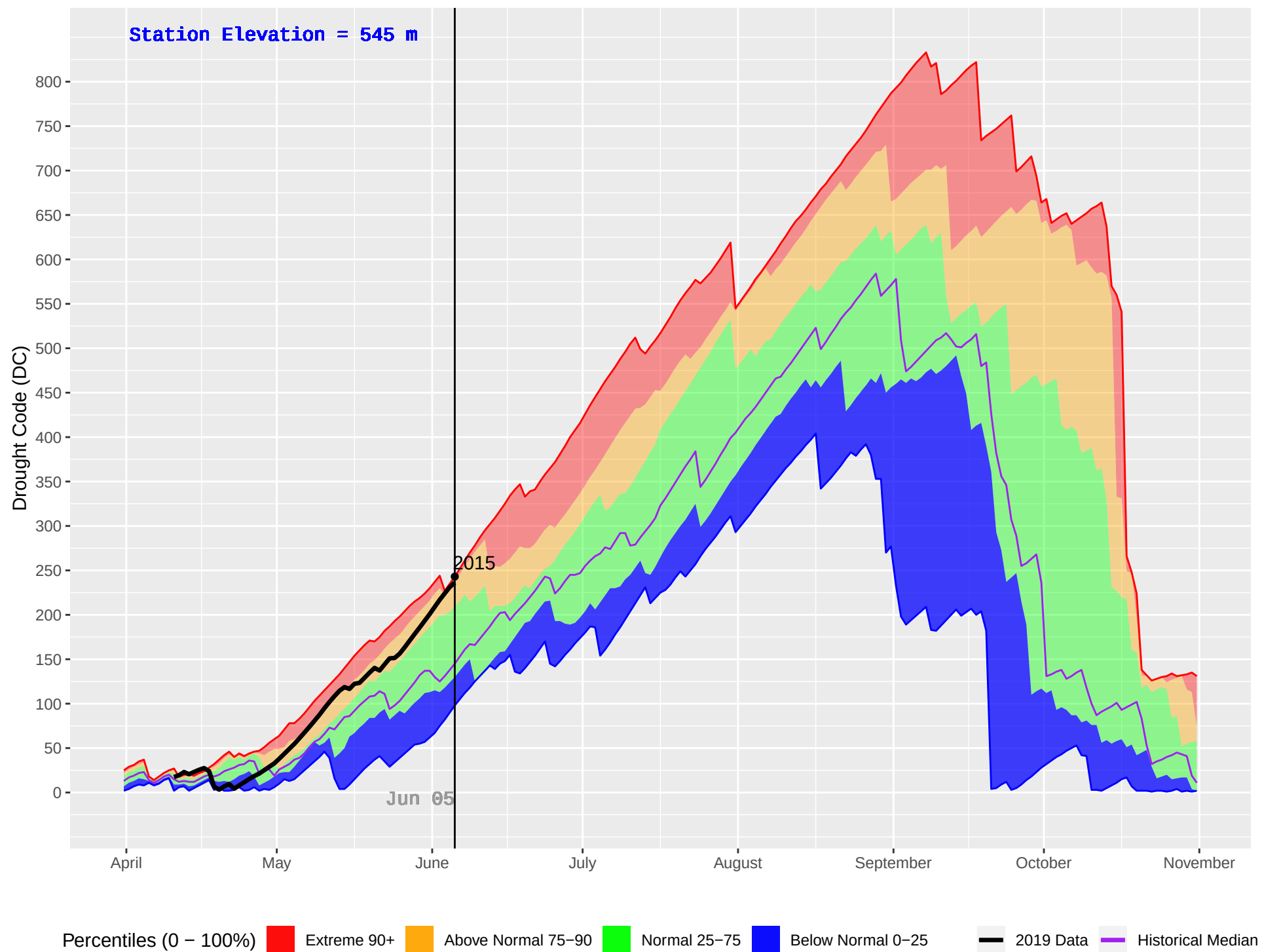
MEAGER CREEK (1083) : Historical (2010–2018) and Current (2019) Daily Drought Code (DC)
