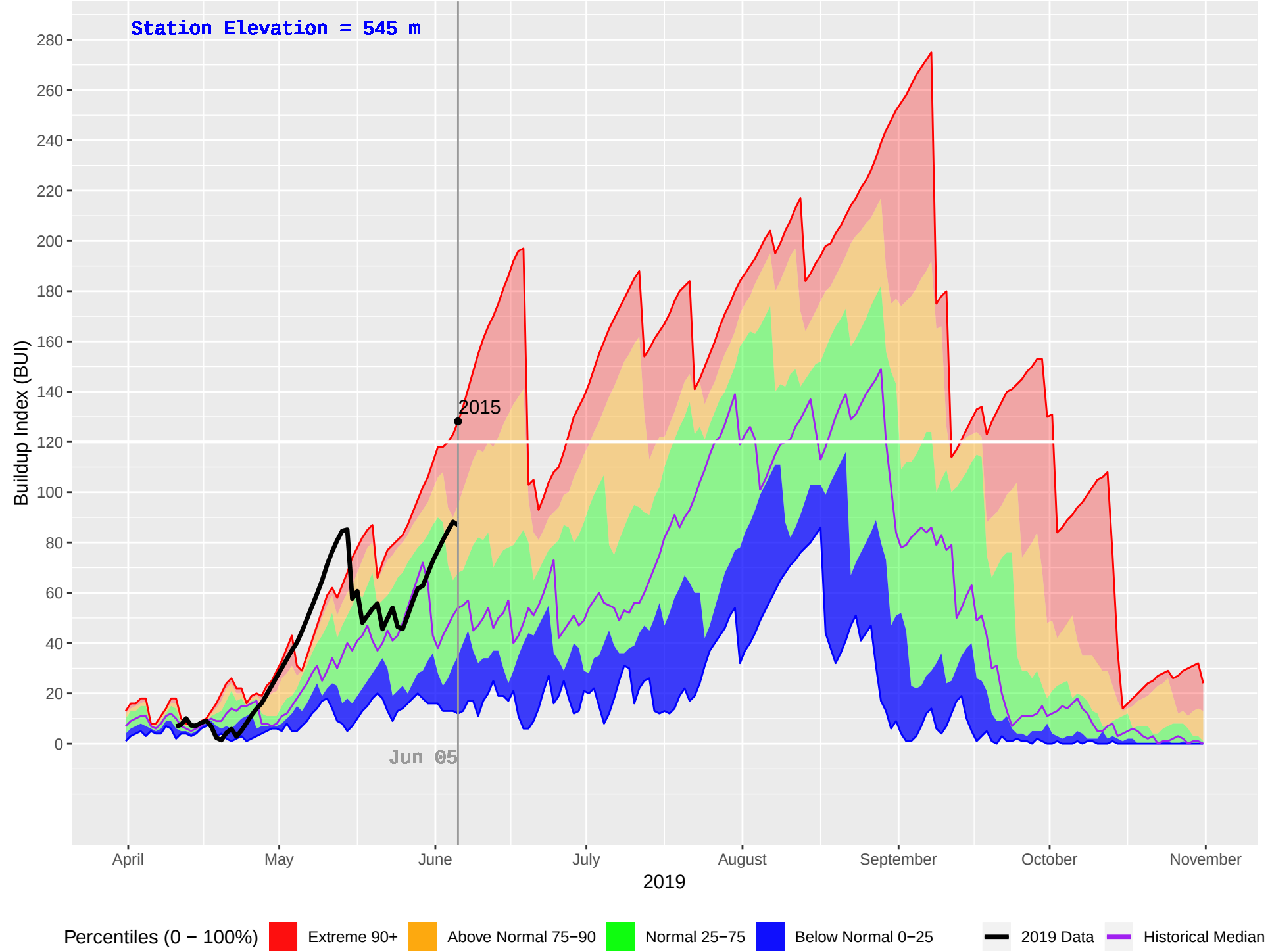
MEAGER CREEK (1083) : Historical (2010–2018), Current (2019) Daily Buildup Index (BUI)
