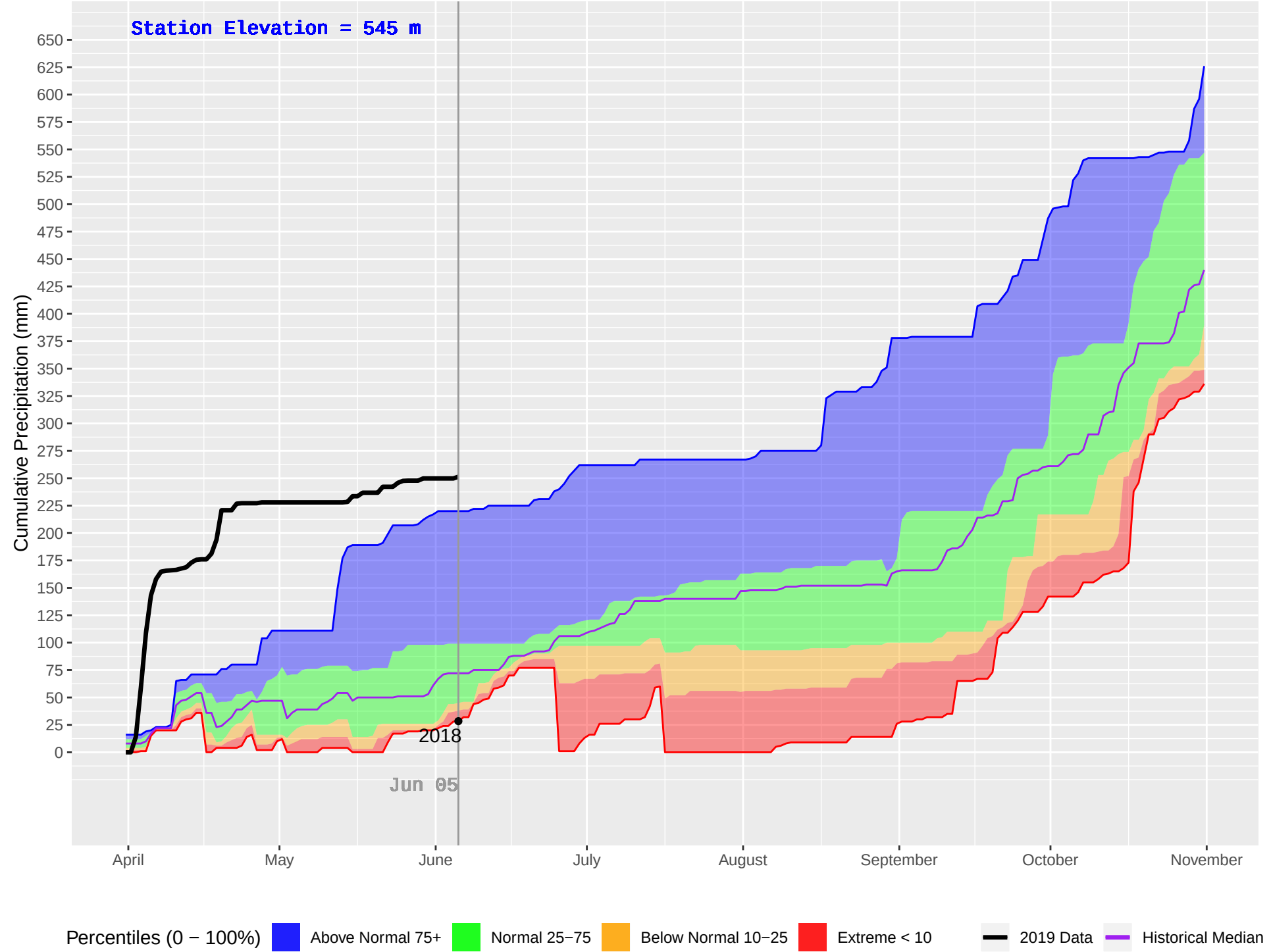
MEAGER CREEK (1083) : Historical (2010–2018), Current (2019) Daily Cumulative Precipitation
