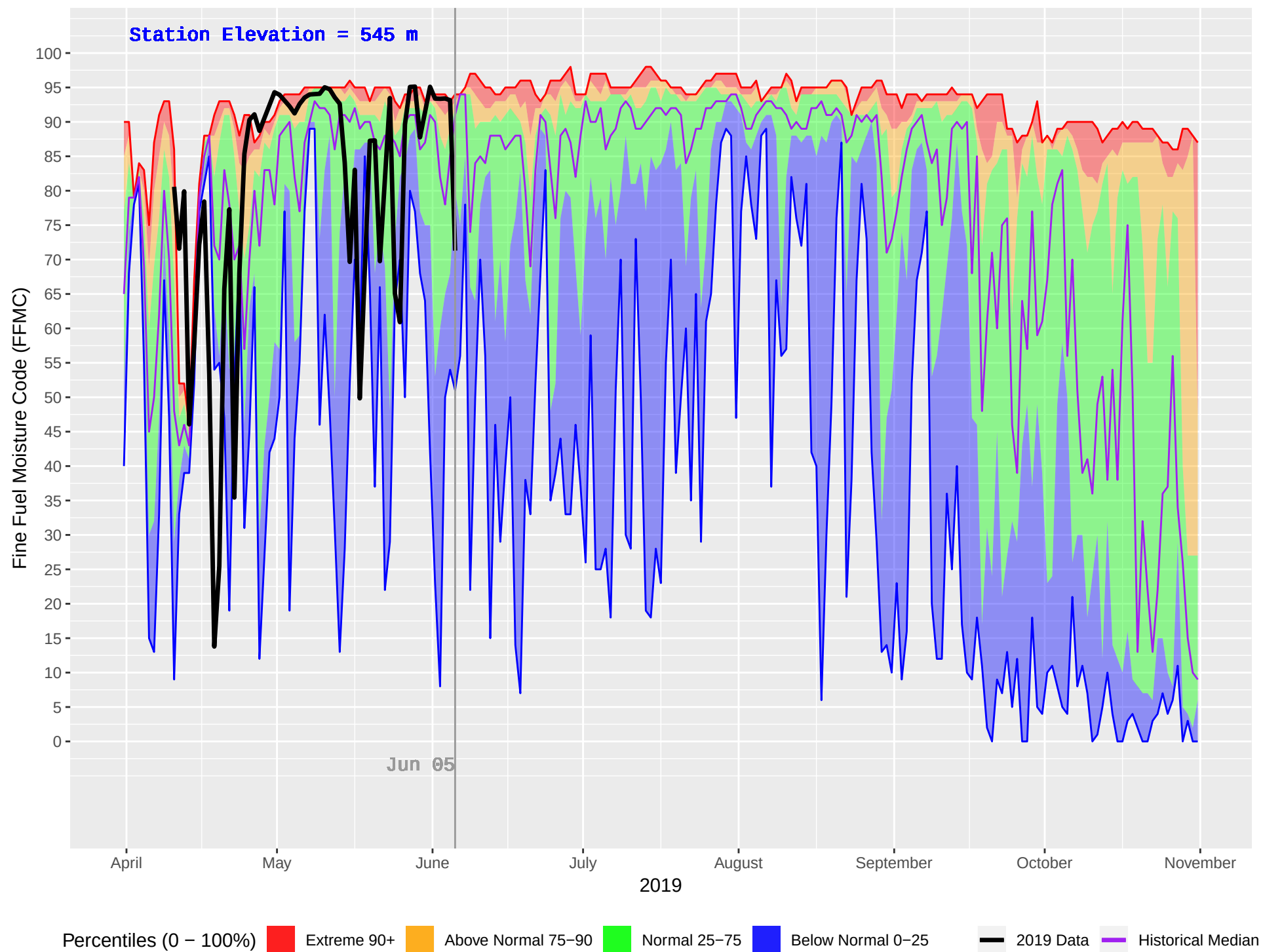
MEAGER CREEK (1083) : Historical (2010–2018) and Current (2019) Daily Fine Fuel Moisture Code (FFMC)
