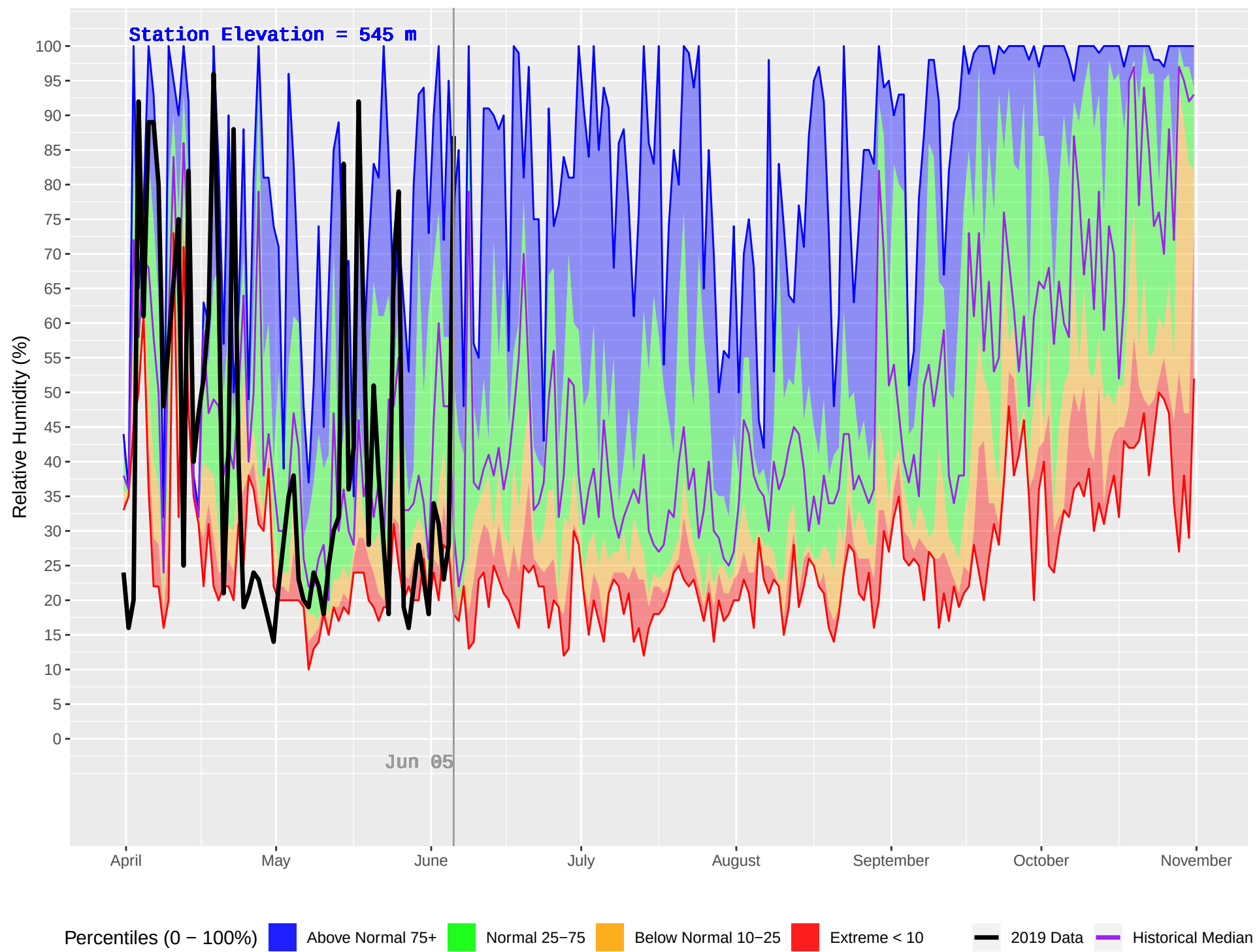
MEAGER CREEK (1083) : Historical (2010–2018) and Current (2019) Daily Relative Humidity
